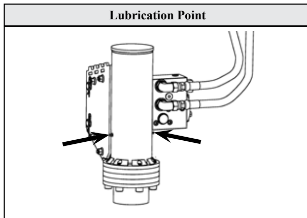
Left & Right Sides of Unit - 2 Zerks
