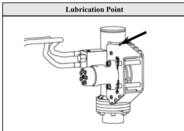
Top Back Side of Unit - 1 Zerk
